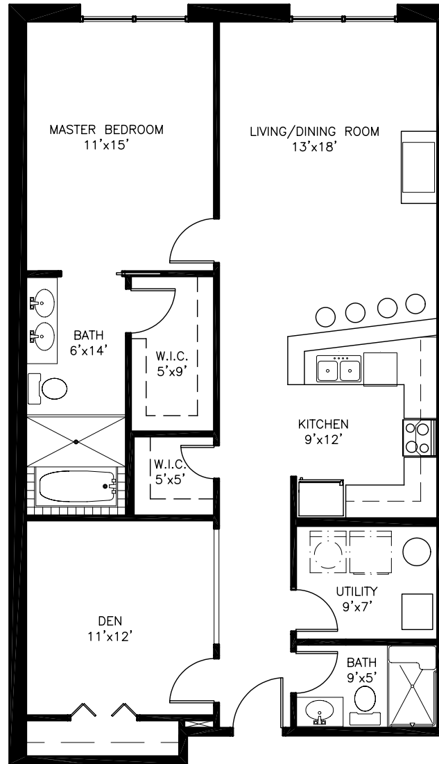
1 UNIT #1 FLOOR PLAN UNITS # 201, 301 & 401 - 1130 SQ. FT. (EACH)
